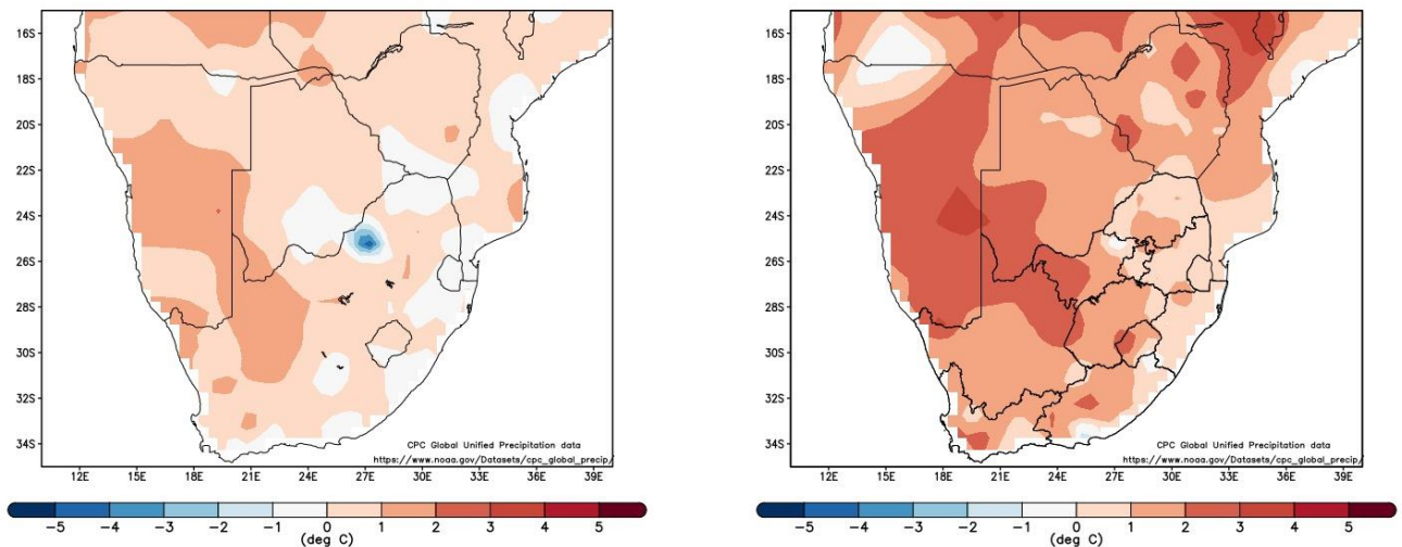
Figure 9: Composite minimum and maximum temperature anomaly for NDJ 2023/2024
