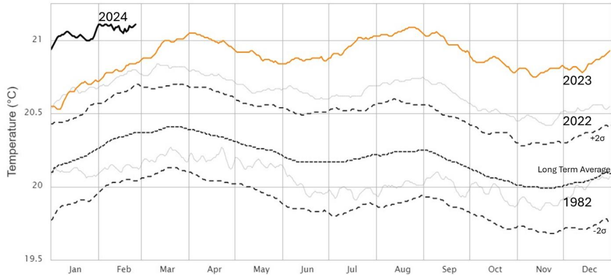
Figure 2: Global average SSTs for selected years showing relative changes and trends. Adapted from Climateanalyzer.org. The bimodal distribution of these data are related to a range of seasonal physical processes.
